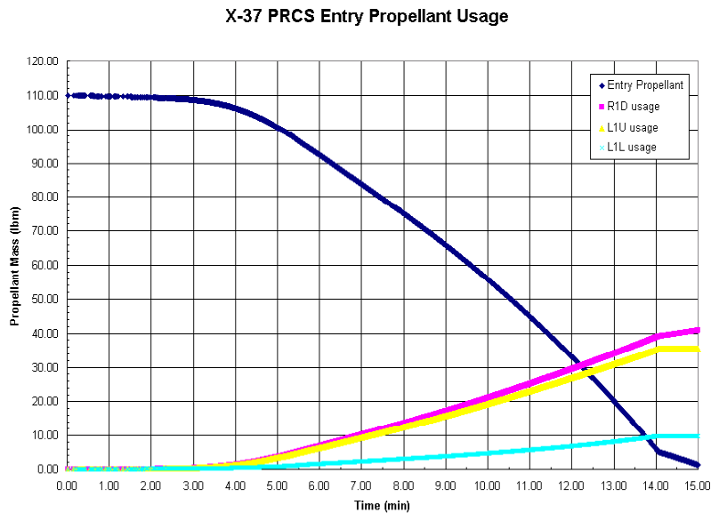
Figure 11 PRCS Entry Propellant Usage.
