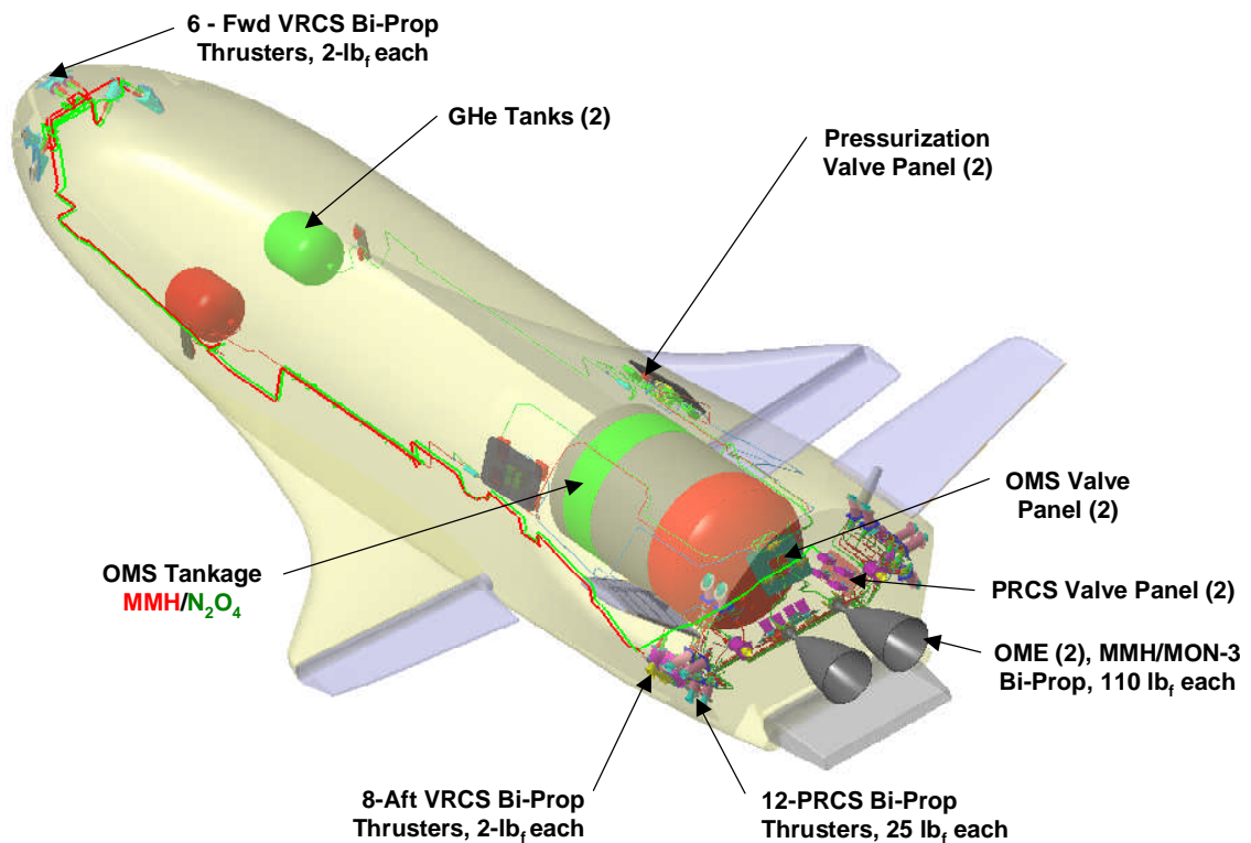
Figure 4 System Configuration.
