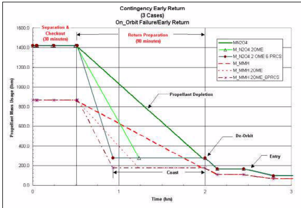
Figure 9 Contingency Early Return.
