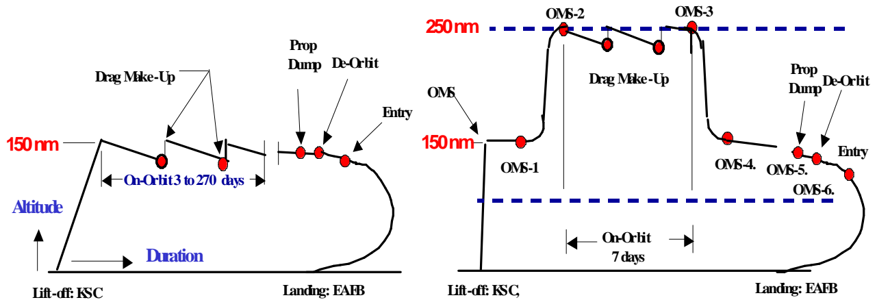
Figure 8 X-37 Design Reference Missions.
