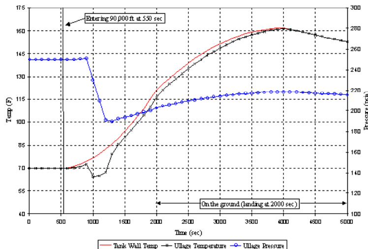
Figure 12 Re-Entry Venting.
