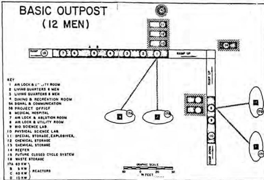
Fig. I-4. Layout of Basic 12-Man Outpost
